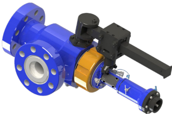
CX-HB3.0 Hydra-Balanced Choke with optional gantry installed
